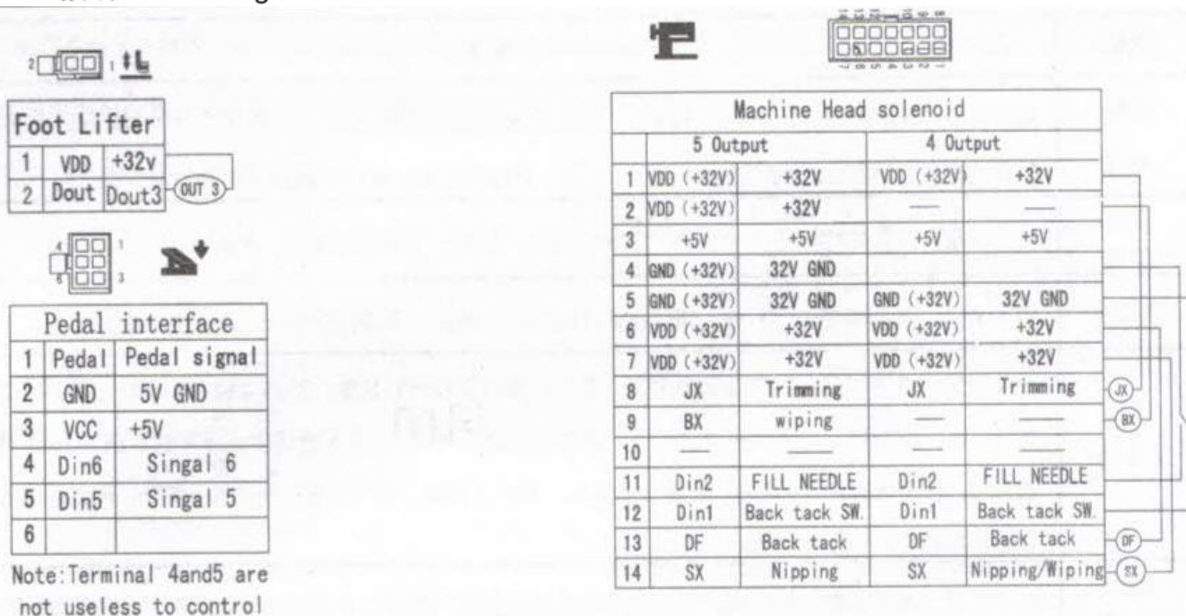
Fig.1-2 Controller Interface Definition
