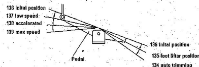
Fig. 4-1 pedal movement of each position parameter
